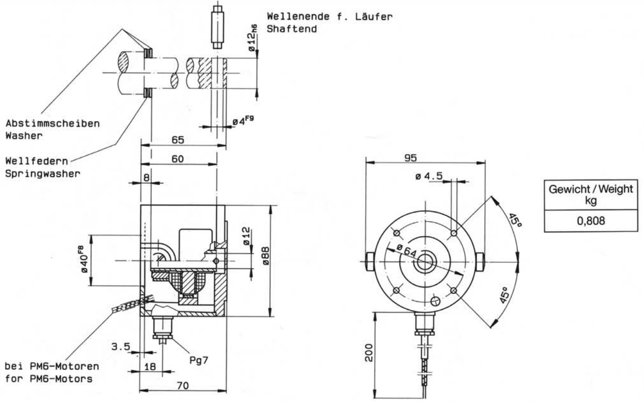
Maße ohne Toleranzangabe unverbindlich / Dimensions are in mm and are for reference only
